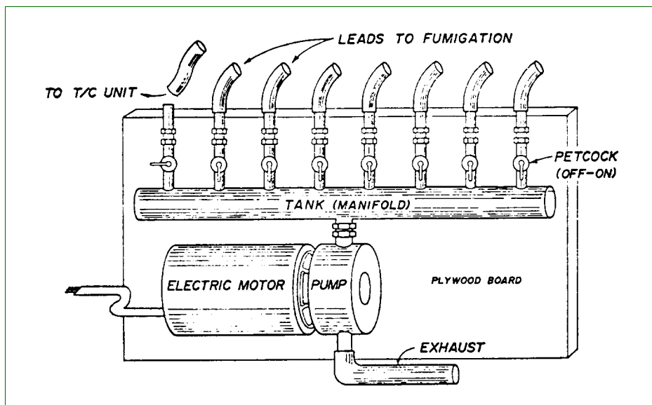
Figure 8-1-6 Auxiliary Pump
